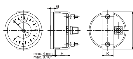
7119 U-clamp steel, zinc plated
