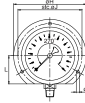
7112 backflange st. steel
