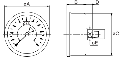
7014 centerback
